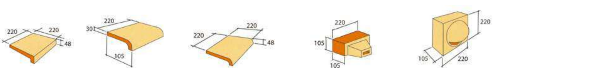
93 - Sill 48 - Cownose sill brick 116 - Bullnose sill 248 - Gargoyle 128 - Ventilation Shell
