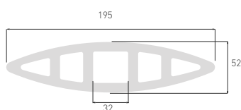
BO-200x50
